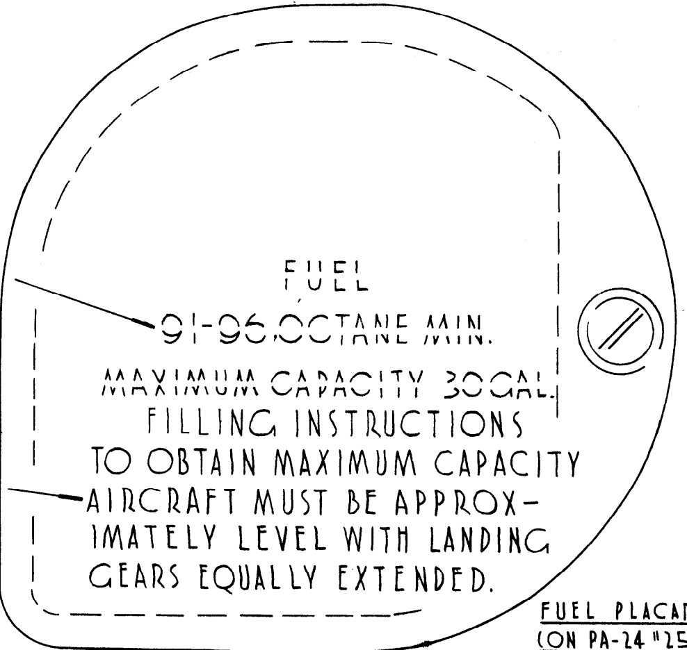
FUEL PLACARD DETAIL (ON PA-24 ONLY)
