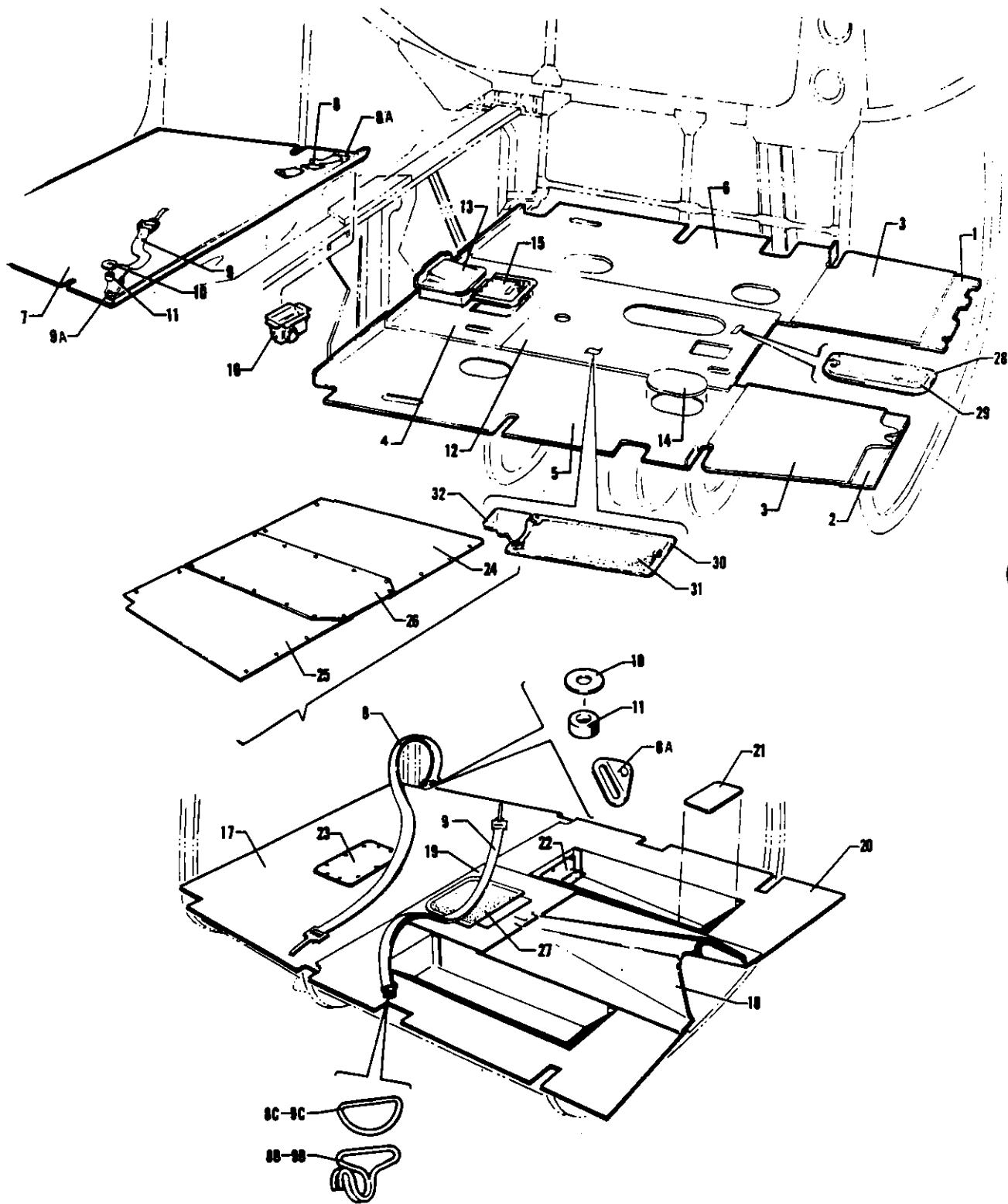
Figure 9. Floorboard Installation
