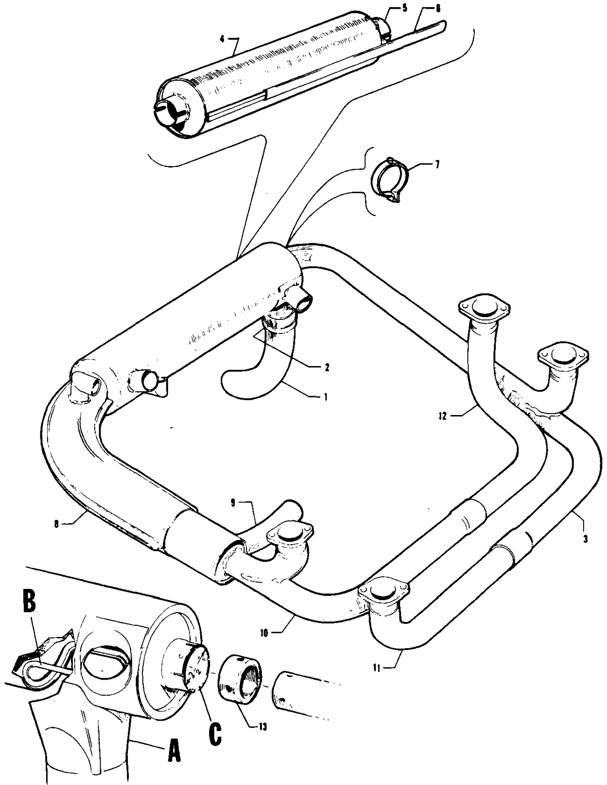
Figure 27. Engine Exhaust Installation "180"
