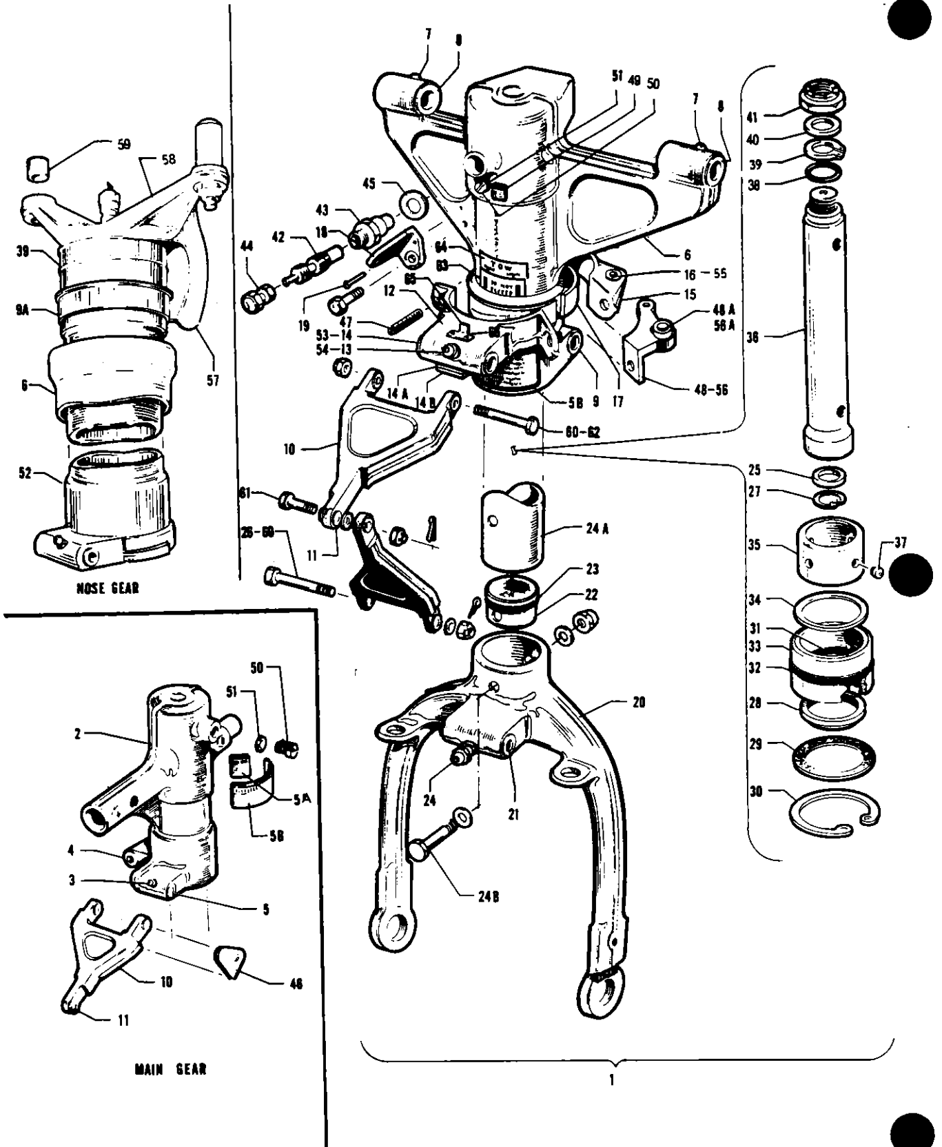
Figure 19. Landing Gear Strut Assemblies "180" & "250"
